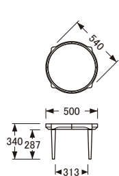
[50φ×H34]
